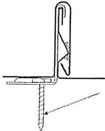
IL20 SEAM PROFILE
