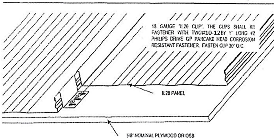
IL20 ASSEMBLY ISOMETRIC
