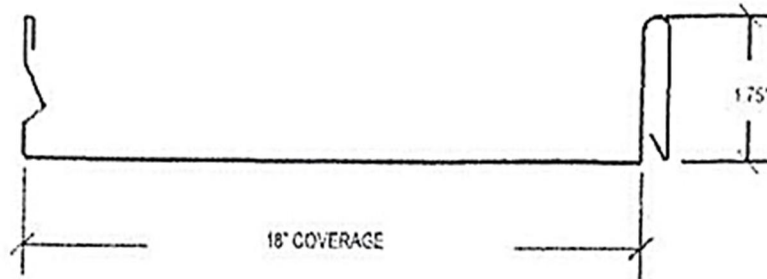
IL2018 PANEL PROFILE
